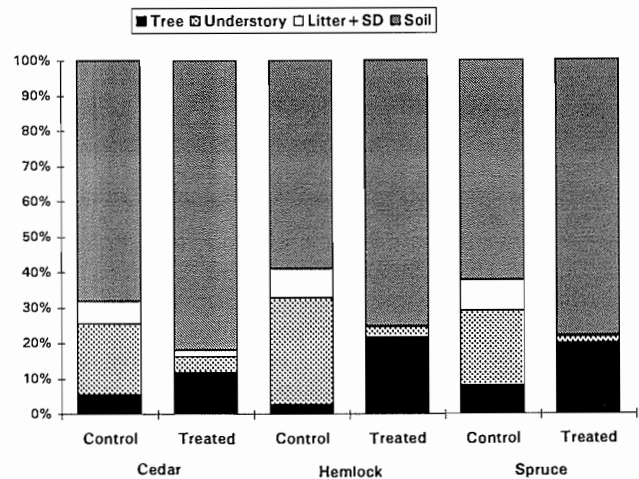
Fig. 1. Distribution of ^{15}\text{N} in the soil-plant systems expressed as a percentage of total applied ^{15}\text{N} recoveries. SD, standing dead. Litter is total plant litter (tree + understory).
